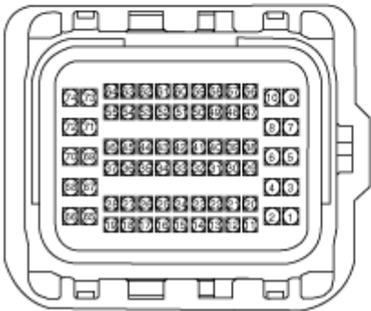
[TCM Connector]
