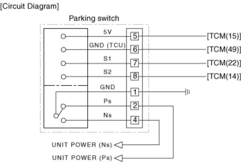
[Connector]
